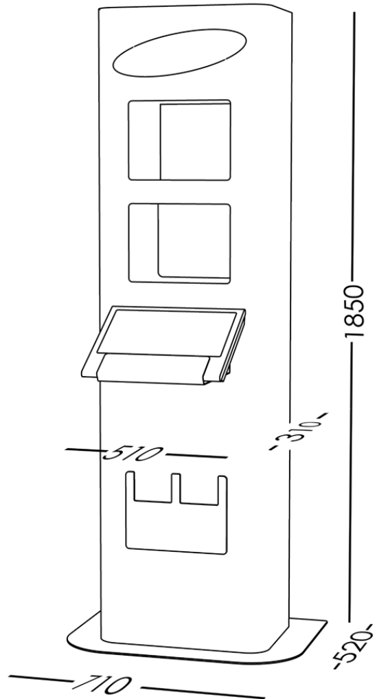
dimension in millimeters
